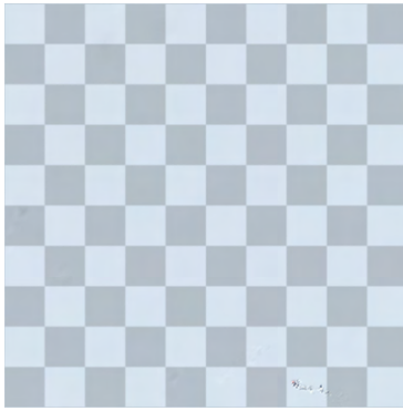
(a) Step 1000
