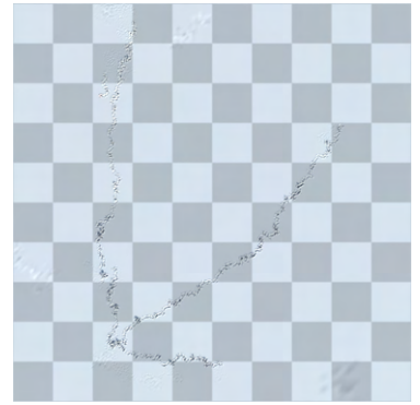
(c) Step 3000
