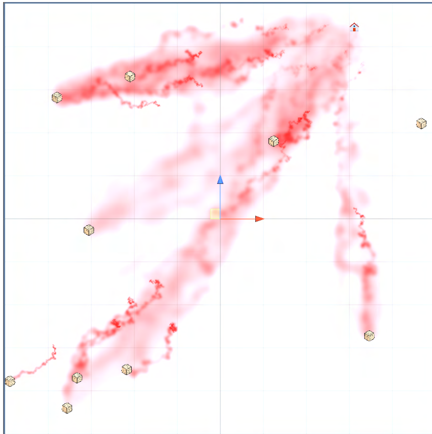
Figure 3.2: Image depicting pheromone concentration on the terrain with heightmap display disabled. Sugar cubes represent food across the landscape with the home icon representing the ants' colony. A white-to-red gradient is used to showcase the respective low-to-high pheromone concentration.
