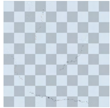
(c) Step 3000
