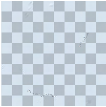
(a) Step 1000
