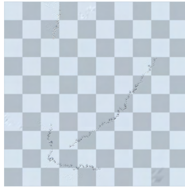
(b) Step 2000
