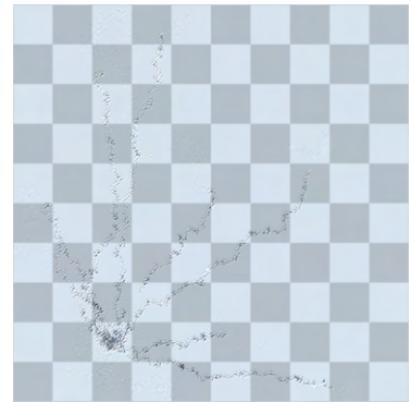
(i) Step 9000
