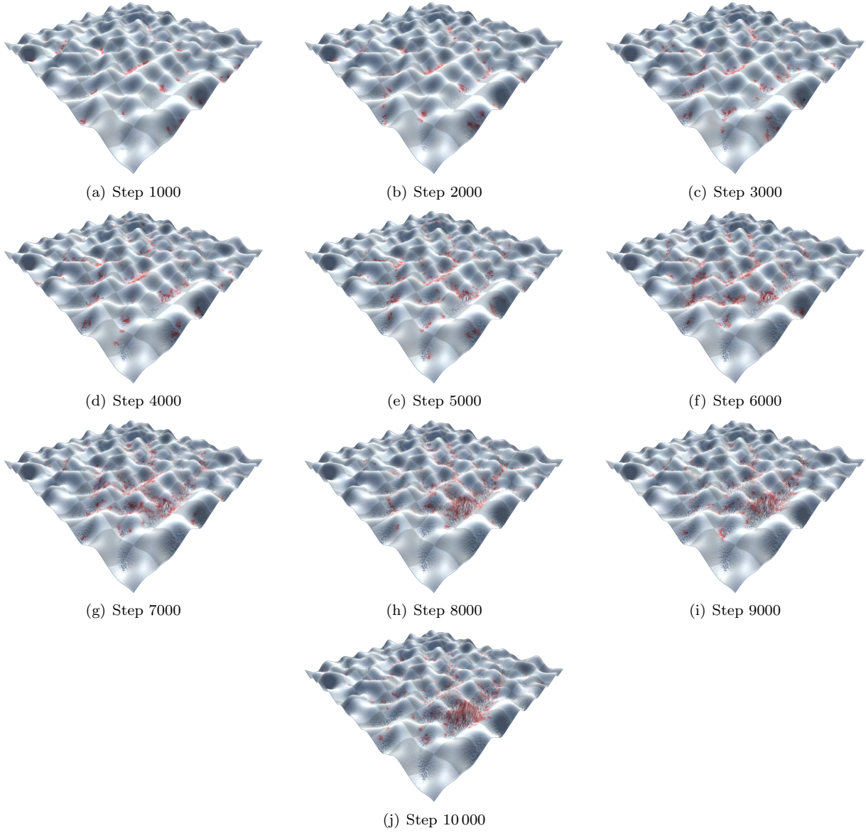
Figure 4.6: Experiment 615's progressive visualization derived from ant movements after 10 000 iterative steps.
