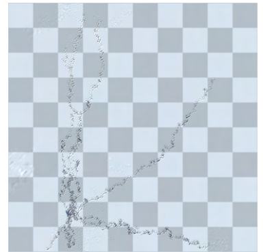
(i) Step 9000
