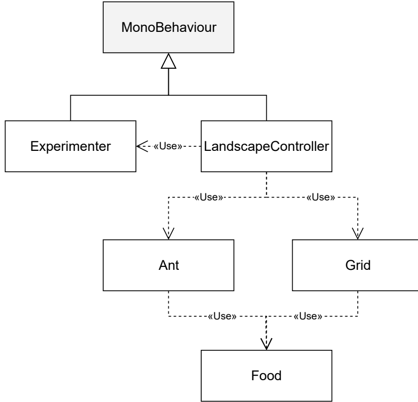
Figure 3.3: Simple UML class diagram representing the project’s structure. MonoBehaviour is a Unity class.
