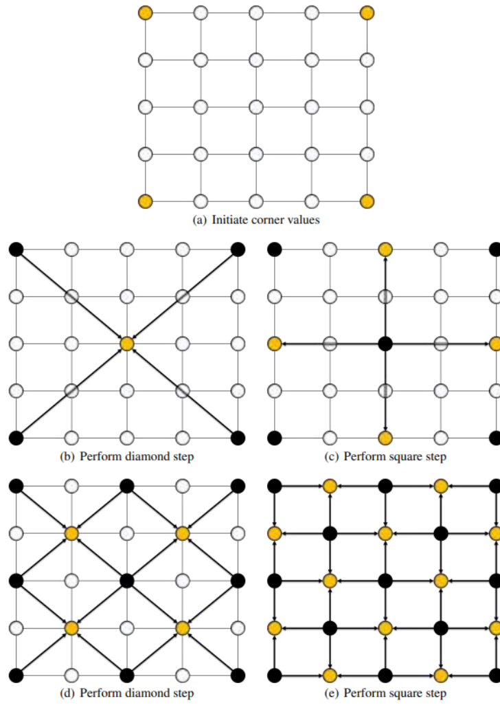
Figure 2.3: Procedure for the Diamond-Square algorithm in 5 steps. Source: Yannakakis & Togelius [40].
